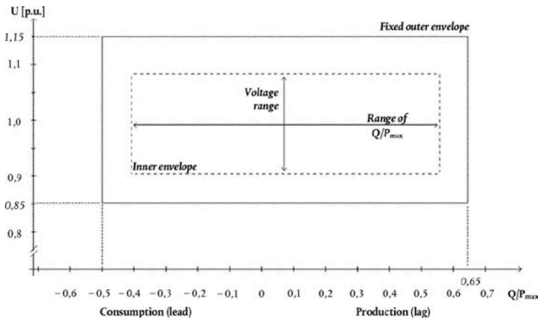
Figure 7: U-Q/P max -profile of a DC-connected power park module at the connection point. The diagram represents boundaries of a U-Q/P max -profile of the voltage at the connection point[s], expressed by the ratio of its actual value to its reference 1 pu value in per unit, against the ratio of the reactive power (Q) to the maximum capacity (P max ). The position, size and shape of the inner envelope are indicative and other than rectangular may be used within the inner envelope. For profile shapes other than rectangular, the voltage range represents the highest and lowest voltage points. Such a profile would not give rise to the full
